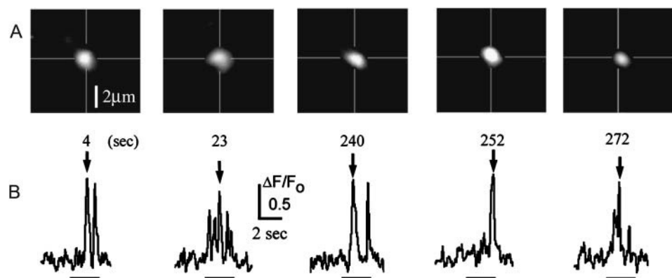
FIGURE 7 N-type \text{Ca}^{2+} channels are anchored in the oocyte membrane. Data were obtained from an oocyte stimulated by two trains of depolarizing pulses ( -15 mV, train of five 3-s depolarizations at 0.1 Hz) separated by an interval of \sim 4 min. (A) Representative images of sparklets arising at a single channel at various times as indicated. Cross-hairs mark the initial position of the sparklet centroid. (B) Traces show fluorescence measurements throughout corresponding depolarizing pulses obtained from a region of interest (1 \mu\text{m}^2 ) centered on this channel.
