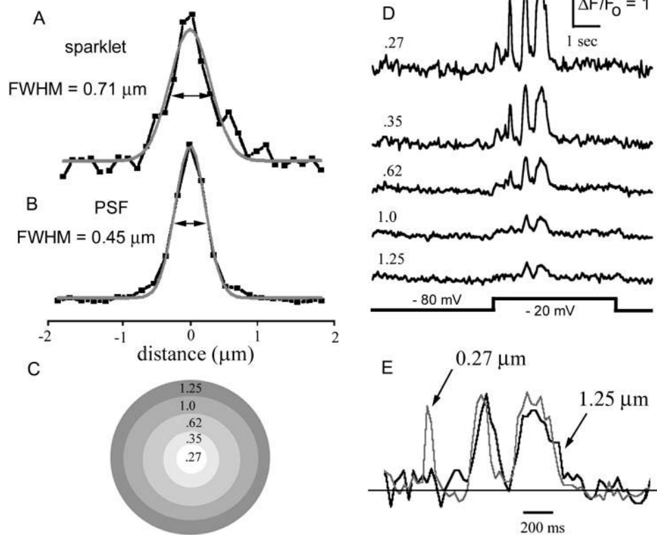
FIGURE 6 Spatial spread and kinetics of fluorescence signal during sparklets. (A) Radial distribution of fluorescence intensity across the sparklet. Dark trace shows the mean of fluorescence measurements made across a line (width 0.5 \mu\text{m} ) passing diametrically through images of nine sparklets, each captured as a single video frame at the time of peak fluorescence. Shaded curve is a fitted Gaussian with width (FWHM) = 0.71 \mu\text{m} . (B) Corresponding fluorescence profile and Gaussian fit (FWHM = 0.45 \mu\text{m} ) obtained using a 100-nm diameter fluorescent bead to measure the lateral point-spread function of the microscope. (C) Schematic, illustrating annular regions centered on a channel used to measure the traces in D. Scale corresponds to that in A and B, and numbers indicate mean radial distance (in \mu\text{m} ) of each annular ring from the center. (D) Traces show fluorescence signals measured from these different annular rings during a depolarizing pulse that evoked several sparklets at a single channel. (E) Superposition of records from a spot (0.27 \mu\text{m} radius) centered on the channel and an annular ring of radius 1.25 \mu\text{m} around the channel. Traces are normalized to the same peak value to facilitate comparison of kinetic differences.
